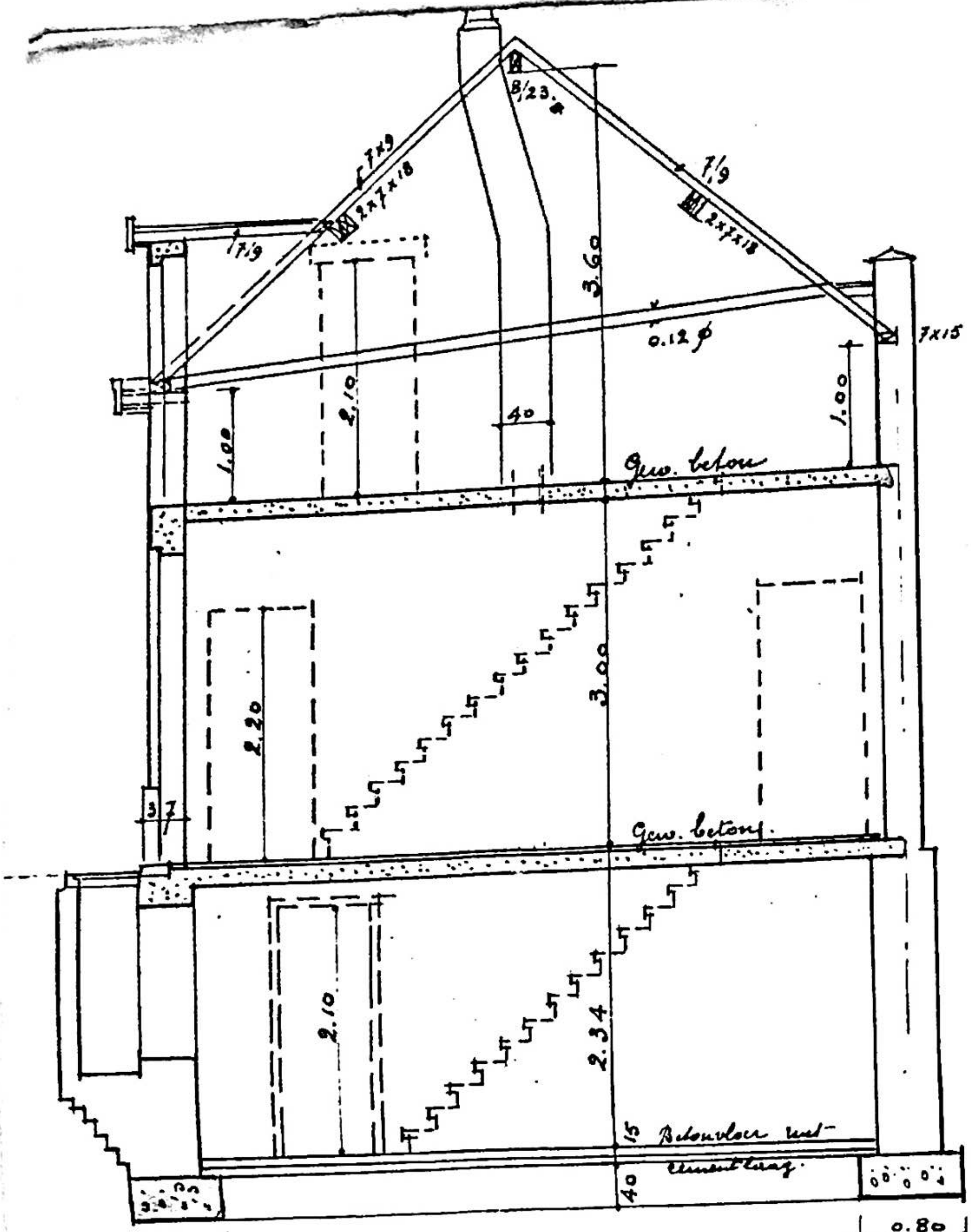
DOORSNED E C.D.
